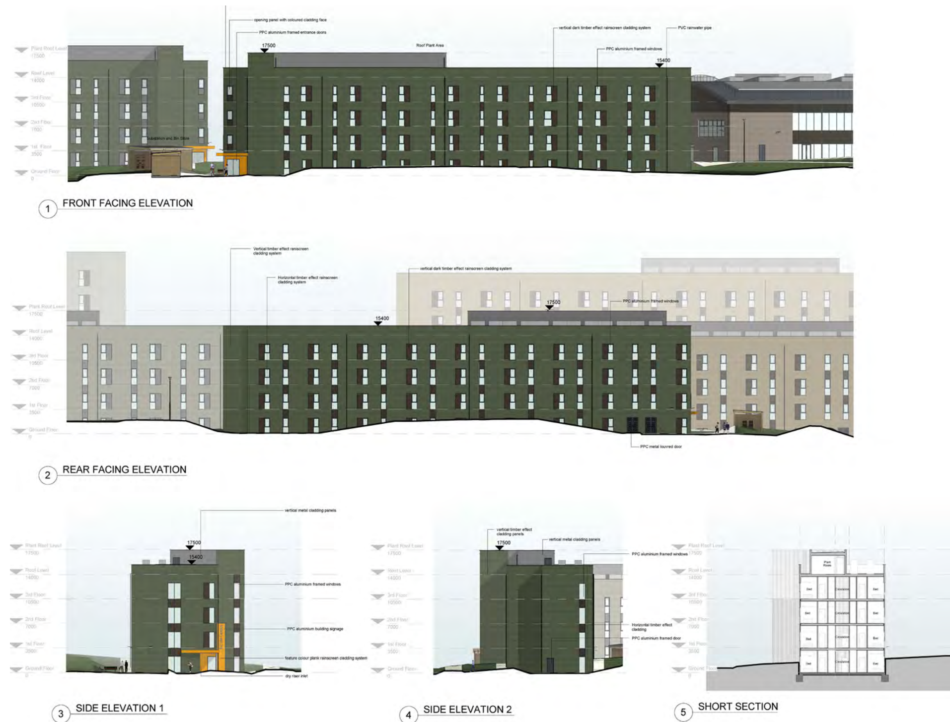
Figure 36 Accommodation buildings sections and elevations
